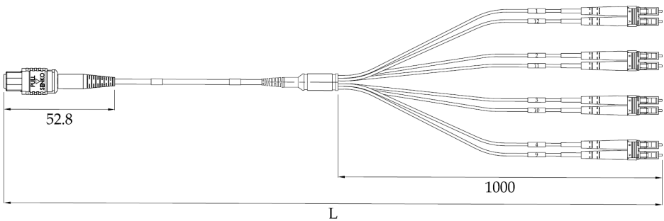
< Female MPO8 to LC, 8 Fibers, 3.0mm >
