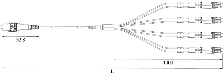
< Male MPO8 to LC, 8 Fibers, 3.0mm >
